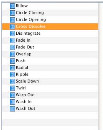
Figure 2. Transitions menu
