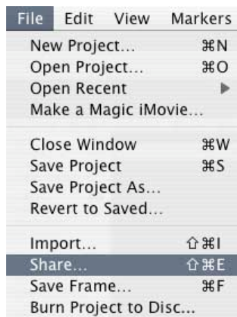
Figure 1. Share option
