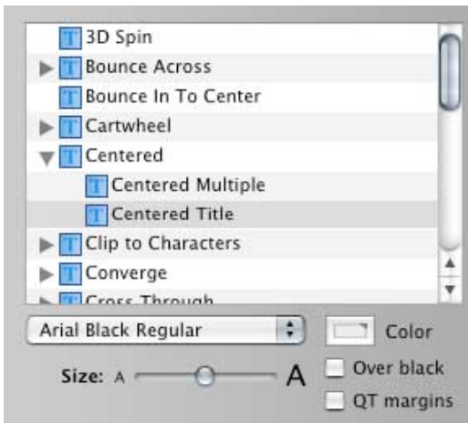
Figure 3. Title Menu
